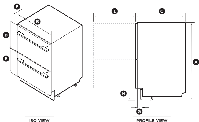
ISO VIEW
