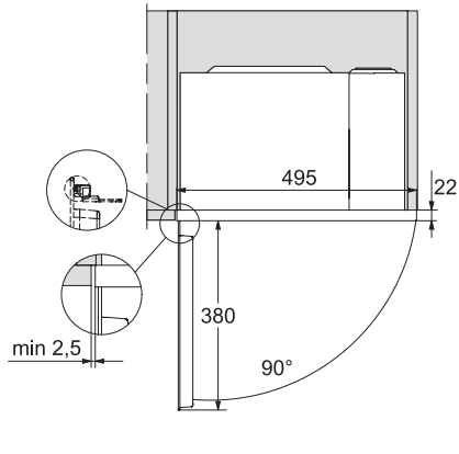
M2224SC, installation drawing
